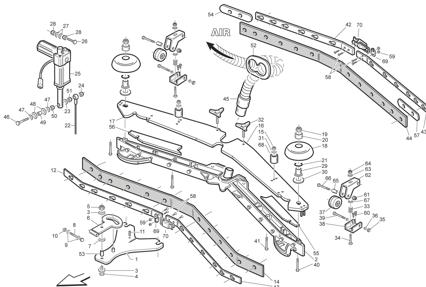
Complete Squeegee Assembly - 3PMVR02004
