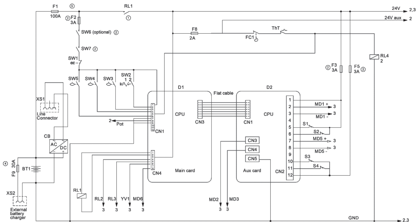
MAIN CONTROL BOARD
